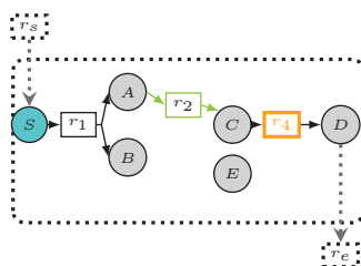
Fig. 12. Topological completion R_1 = \{r_2\} satisfies r_4 \in \text{active}_{G_1}^t(\{S\}) , but carries no flux, due to accumulation of compound B that contradicts equation (6).
