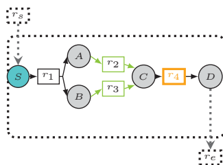
Fig. 11. Completion with the union R_1 \cup R_2 = \{r_2, r_3\} . G = G_1 \cup G_2 satisfies r_4 \in \text{active}_G^h(\{S\}) and thus is flux balanced.
