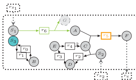
Fig. 4. Solution to metabolic network completion under relaxed stoichiometric activation hypothesis in order to satisfy equations (5)–(9). Notice that within this completed network, there exists no flux distribution allowing the reaction r_5 to be activated.
