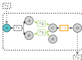
Fig. 14. Completion with the union R_1 \cup R_2 = \{r_2, r_3\} . G = G_1 \cup G_2 satisfies r_4 \in \text{active}_G^t(\{S\}) , but contradicts minimality and carries no flux r_4 \notin \text{active}_G^h(\{S\}) , due to accumulation of compound E that contradicts equation (6).
