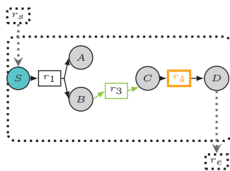
Fig. 10. Topological completion R_2 = \{r_3\} satisfies r_4 \in \text{active}_{G_2}^t(\{S\}) and carries no flux as well, due to accumulation of compound A that contradicts equation (6).
