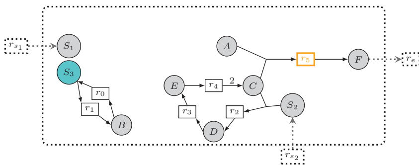
Fig. 1. Example of a metabolic network. Compounds and reactions are depicted by circles and rectangles, respectively. Dashed reactions are reactions involving the boundary between the organism's metabolism and its environment. r_5 is the target reaction. S_1 and S_2 are boundary (and initiation) seeds. S_3 is assumed to be an initiation seed. Numbers on arrows describe the stoichiometry of reaction (default value is 1).
