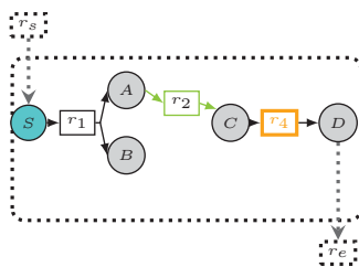
Fig. 9. Topological completion R_1 = \{r_2\} satisfies r_4 \in \text{active}_{G_1}^t(\{S\}) , but carries no flux, due to accumulation of compound B that contradicts equation (6).
